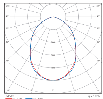
SPMI 240mm 20W 80°:
