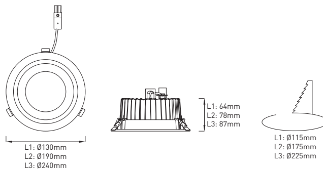
SPMI 130mm 8W 41°:
