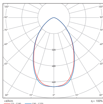
SPMI 130mm 8W 41°:
