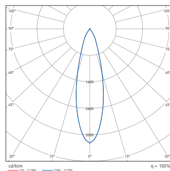
NEMO Surface 4000°K 30°:
